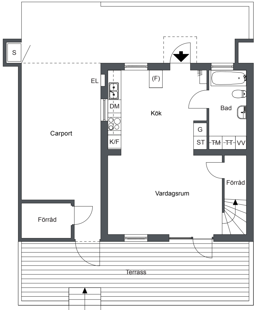
Plan 0
